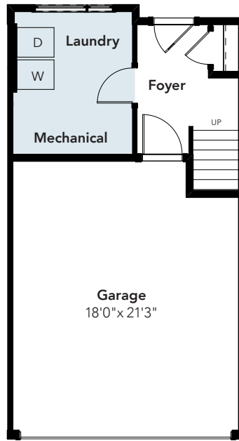
LAUNDRY IN MECH ROOM
