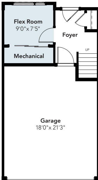
ENCLOSED FLEX ROOM BASEMENT 184 SQ FT
