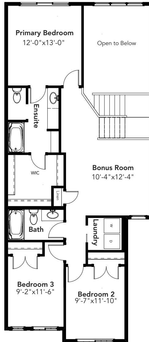
SECOND FLOOR: 1067 SQ FT
