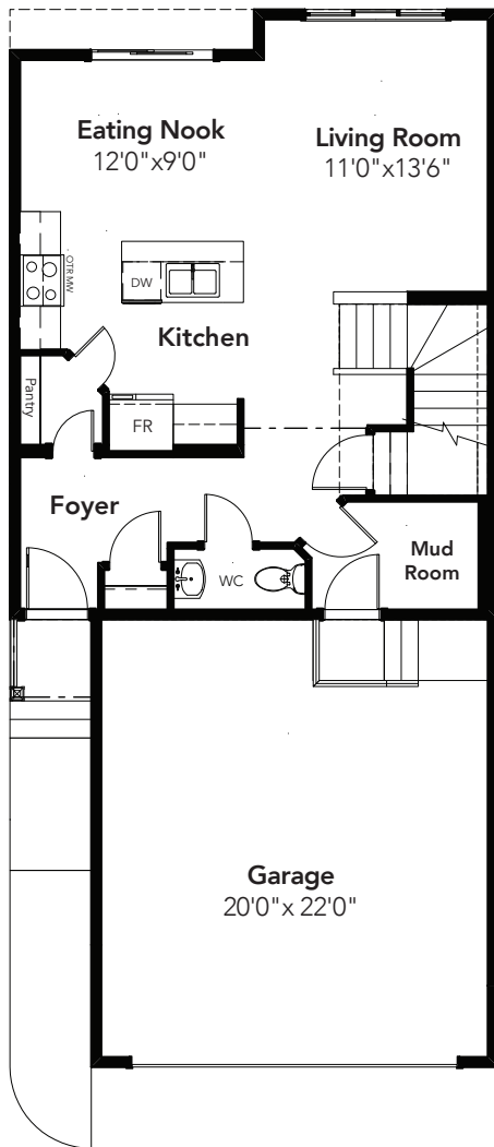
MAIN: 696 SQ FT
