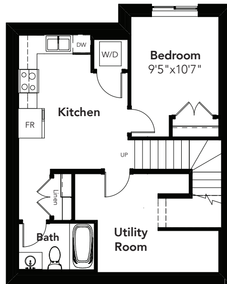
SEPERATE SUITE OPTION BASEMENT: 432 SQ FT
