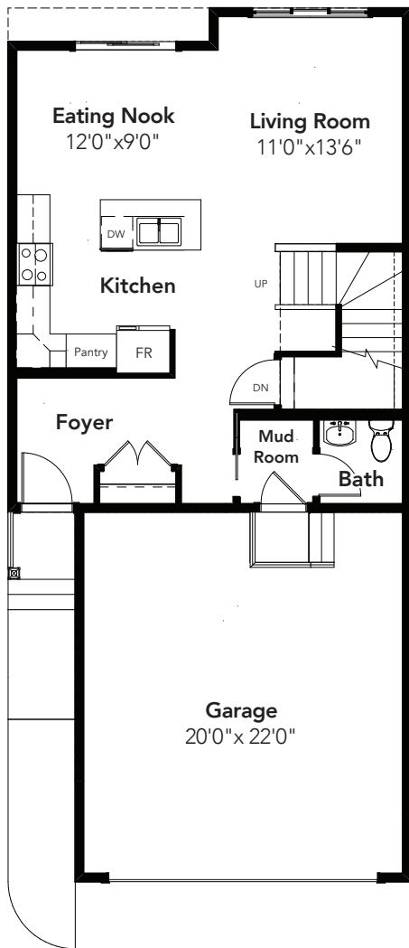
MAIN: CABINET PANTRY OPTION 696 SQ FT
