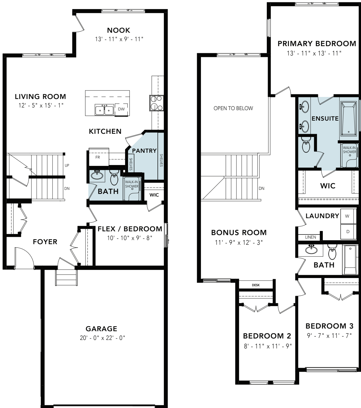
FULL BATH & PANTRY OPTION: 989 SQ FT
