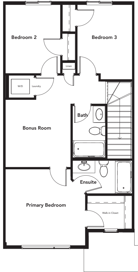
SECOND FLOOR: 726 SQ FT
