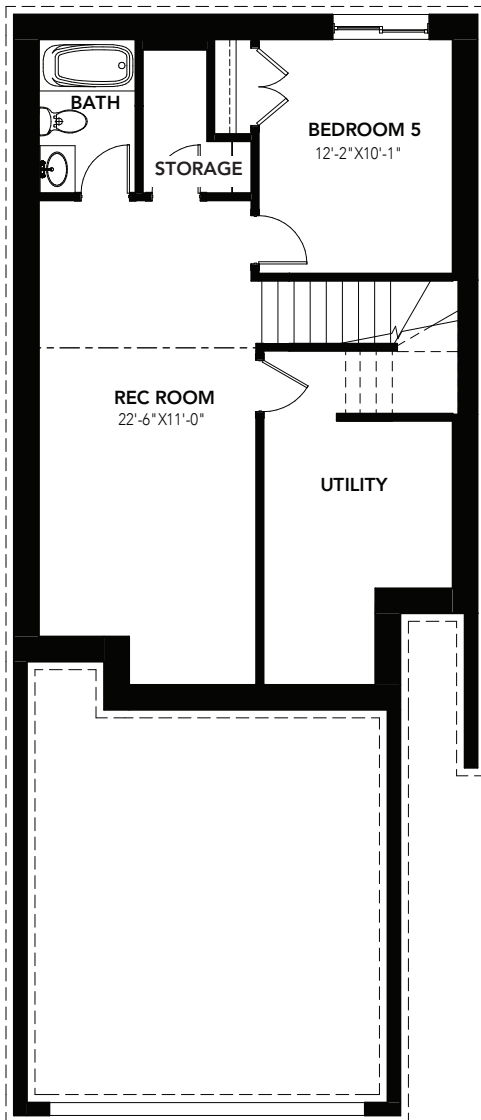
Finished Basement: 498 SQ FT
