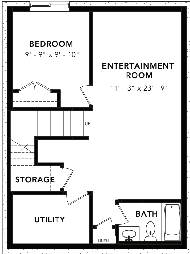
BASEMENT DEVELOPMENT OPTION: 559 SQ FT
