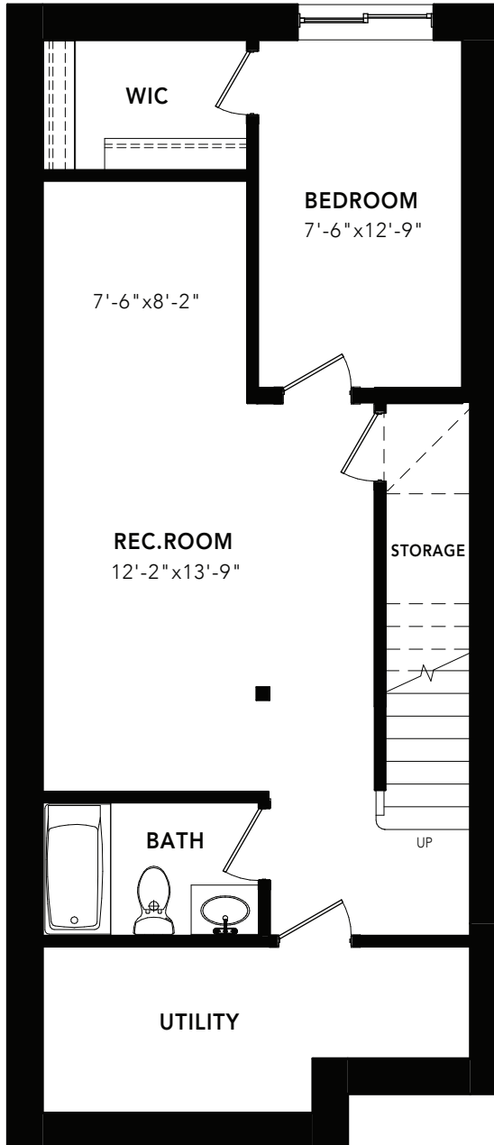
BASEMENT DEVELOPMENT: 474 SQ FT
