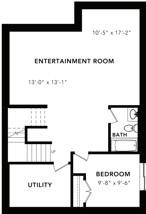
BASEMENT DEVELOPMENT OPTION: 691 SQ FT
