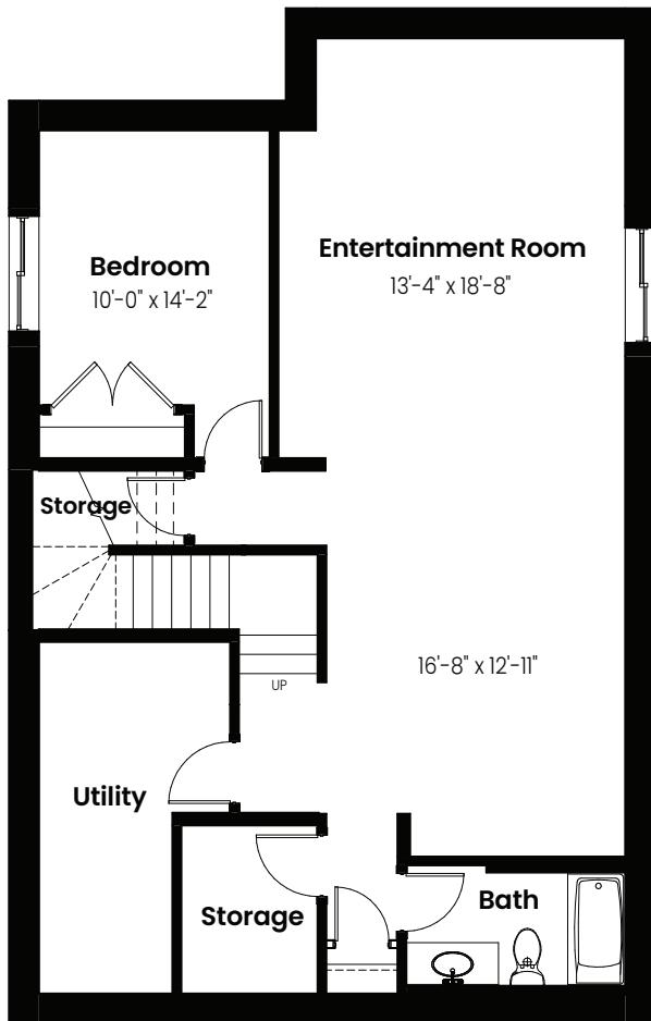
Basement Development Option: 886 Sq Ft
