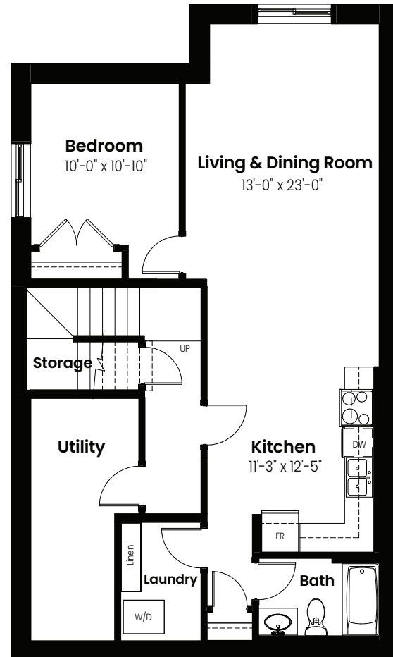
Basement Suite Option: 811 Sq Ft
