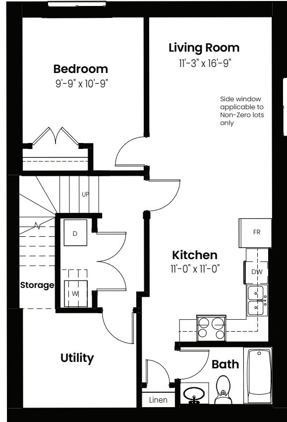
Basement Suite Option: 640 Sq Ft
