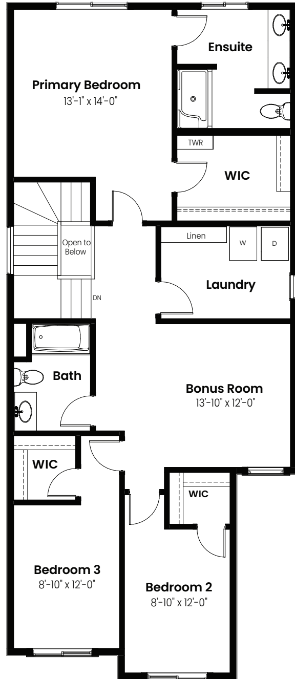
Second Floor: 1230 Sq Ft
