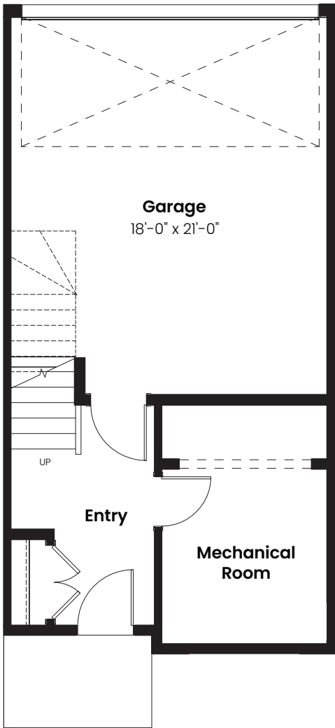
Ground Floor: 119 Sq Ft
