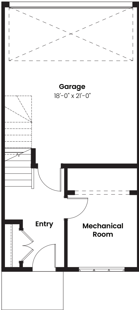
Ground Floor: 127 Sq Ft
